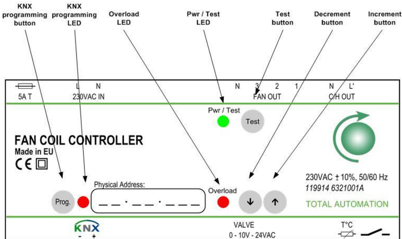
Figure 3: Local push-buttons and LED's
